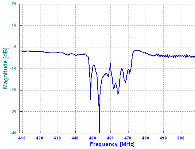
Return Loss
