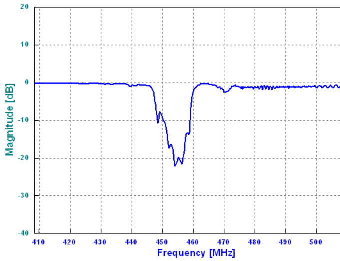
Return Loss
